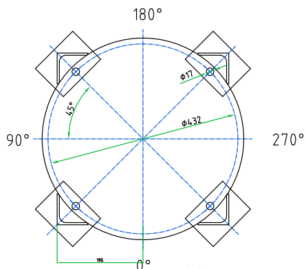
MOUNTING POSITIONS
